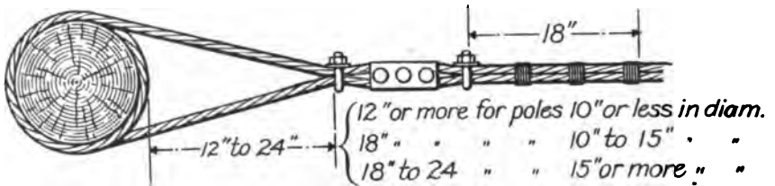
FIG. 133.—Method of dead ending strand.
